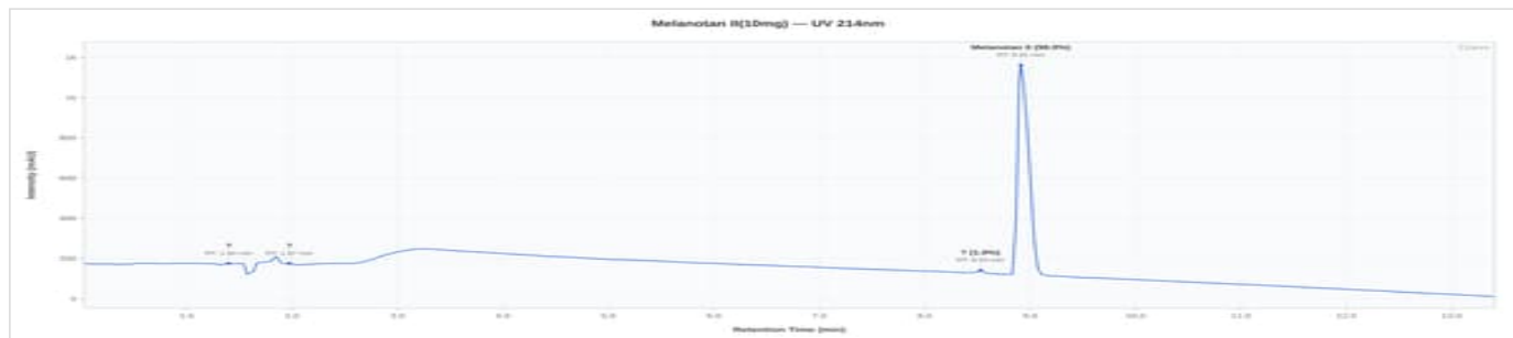
Melanotan II 10mg - MT2-2502-B: UV Chromatogram
